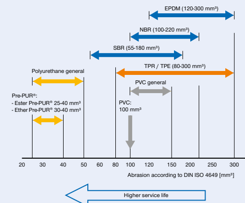
Abrasion resistance
